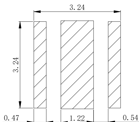
Recommended pad
